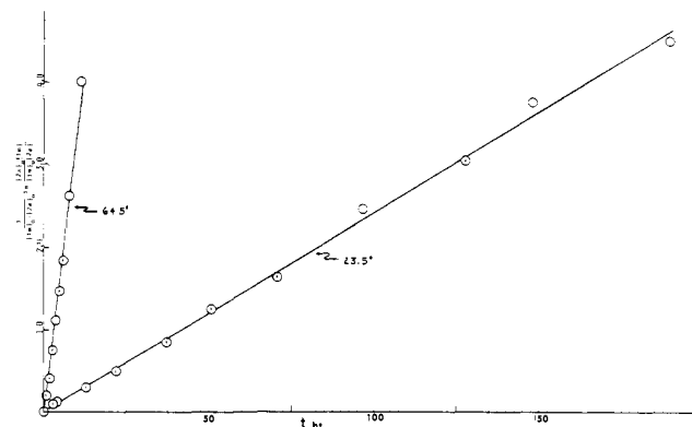
Figure 2. Second-order rate plots for the disappearance of 2a in the presence of Im.
