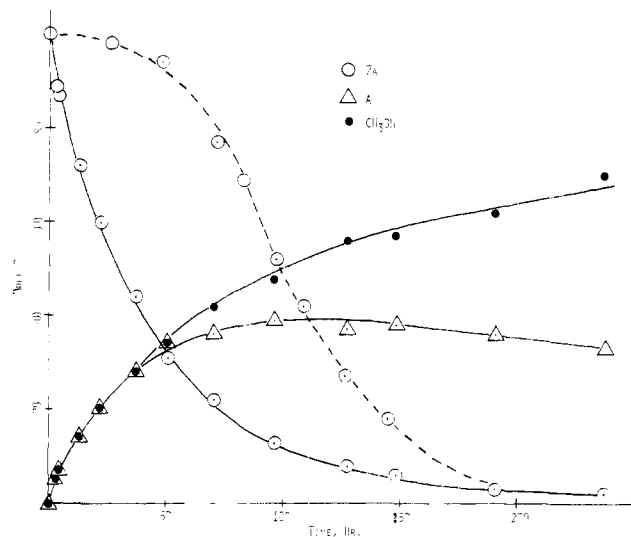
Figure 3. Components of the reaction mixture initially 0.48 M in 2a and 1.14 in M Im in 50% aqueous methanol (deuteriated), as a function of time (23.5 °C).
